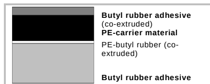
BUTYLEN-N60 and BUTYLEN-S20 design (different thicknesses)
